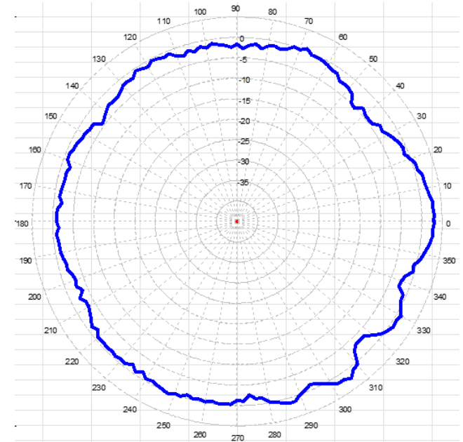
2.5 MHz
