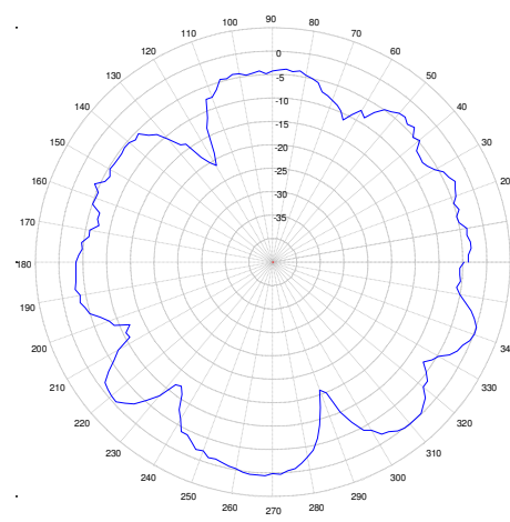
5250 MHz. AZIMUTH
