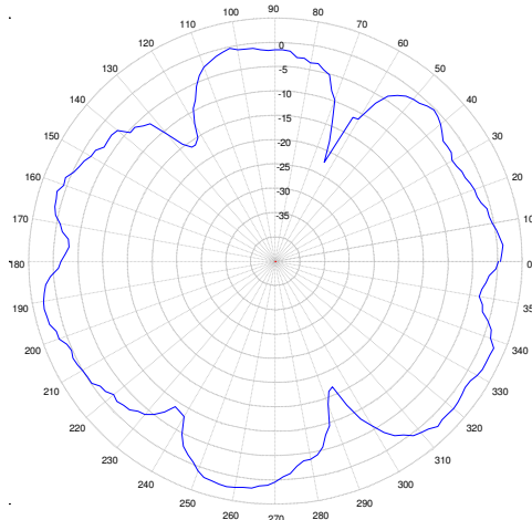
4900 MHz. AZIMUTH
