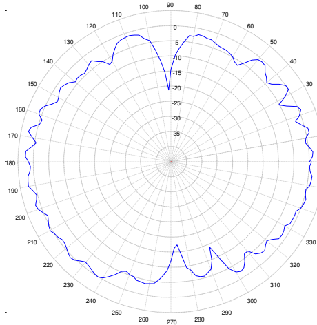
5250 MHz. ELEVATION
