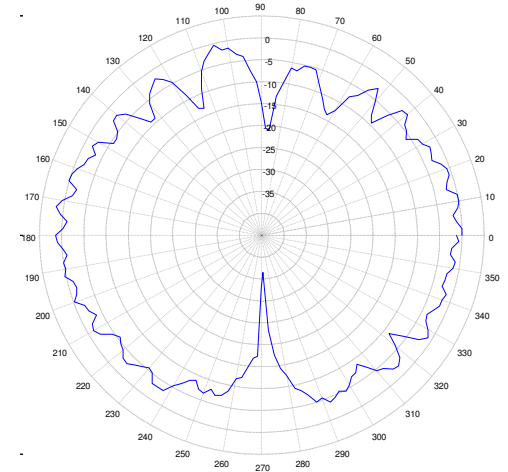
5850 MHz. ELEVATION
