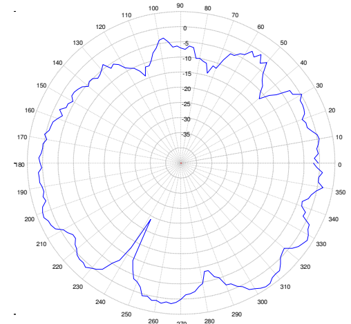
5850 MHz. AZIMUTH
