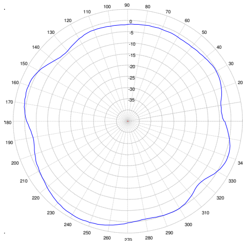
2450 MHz. AZIMUTH
