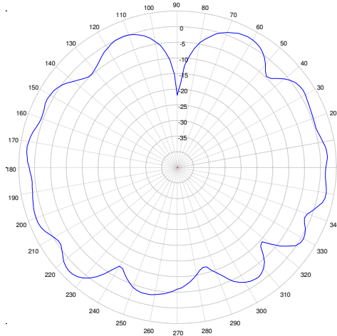
2450 MHz. ELEVATION
