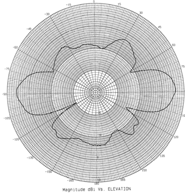
ECOM6-5900 – Elevation Plot
