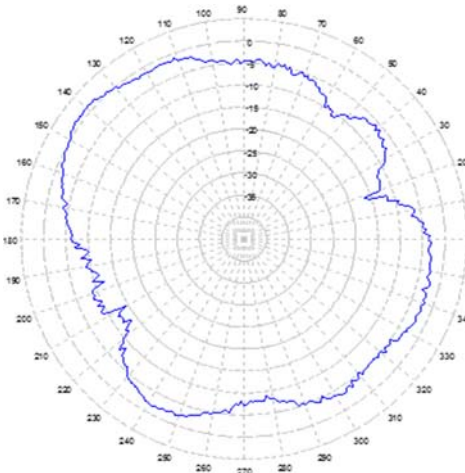
4.9 GHz. AZIMUTH
