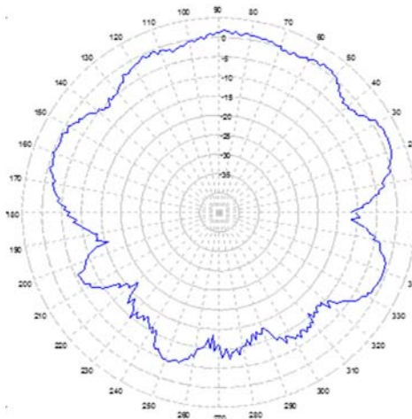
5.35 GHz. AZIMUTH
