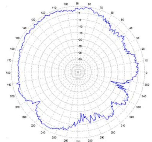
5.85 GHz. AZIMUTH
