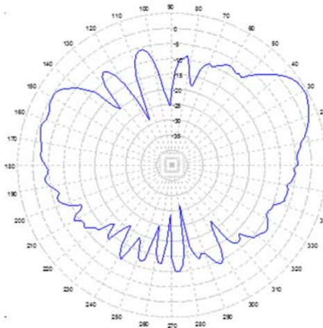
5.35 GHz. ELEVATION
