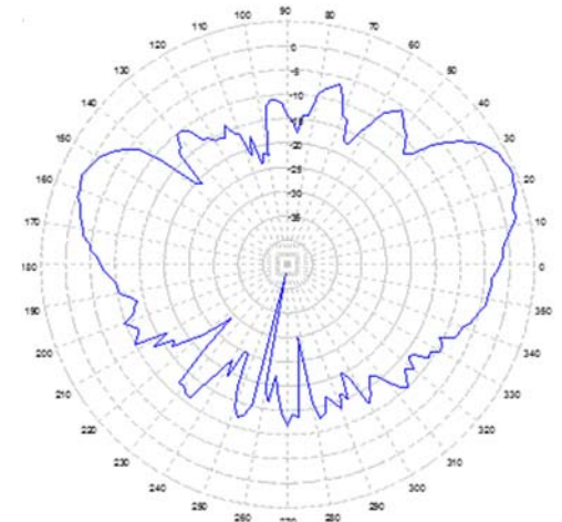
5.85 GHz. ELEVATION
