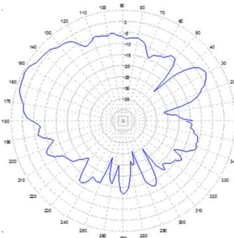
4.9 GHz. ELEVATION
