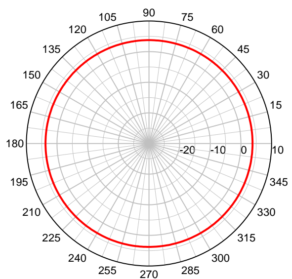
PSKN3-24/55 5-6 GHz – Azimuth Plot
