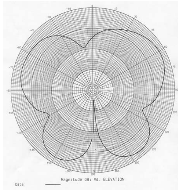
PSTN2 @ 2500 MHz– Elevation Plot
