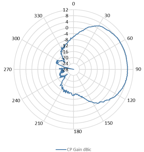
6000 MHz – Azimuth Plot
