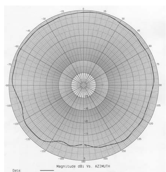
CMD @ 5500 MHz- Azimuth Plot
