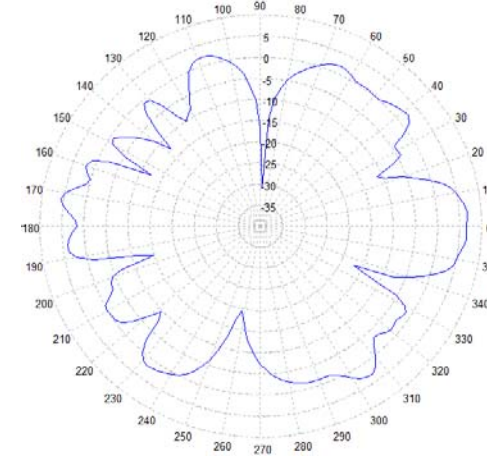
2500 MHz – Elevation Plot
