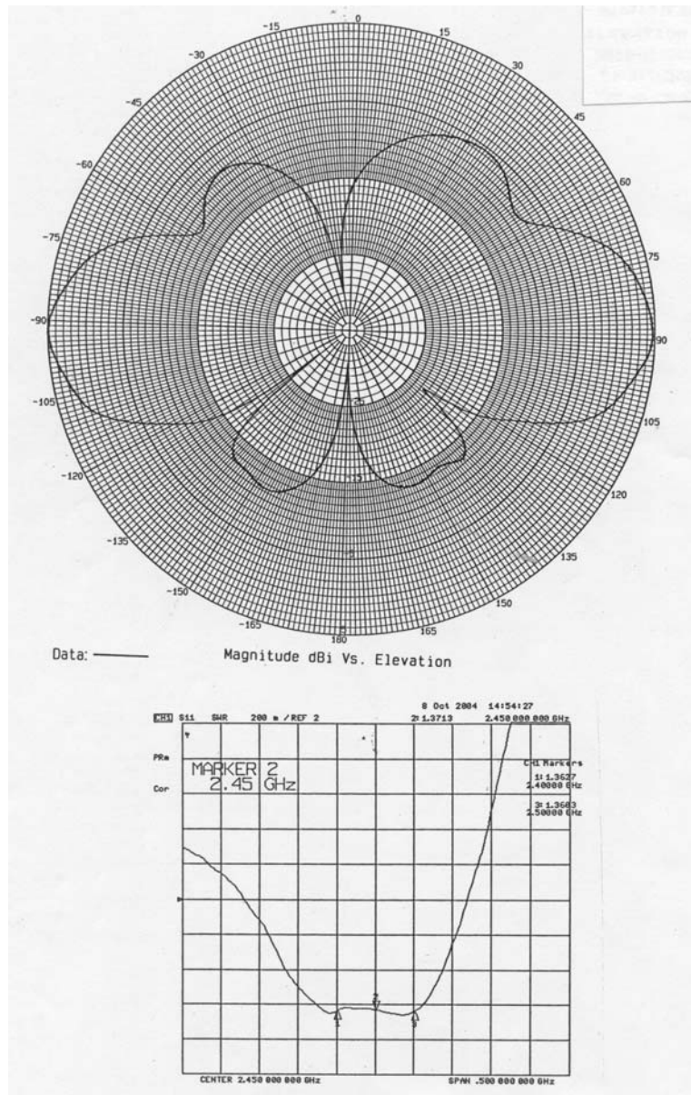
ECOM5-2400 Series – Elevation Plot
