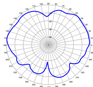
ELEVATION @ 2650 MHz
