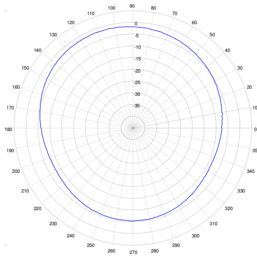
850 MHz. AZIMUTH
