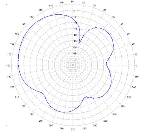
960 MHz. AZIMUTH
