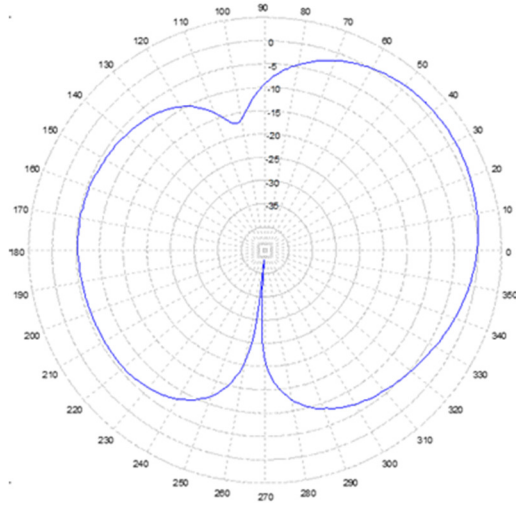
750 MHz. AZIMUTH
