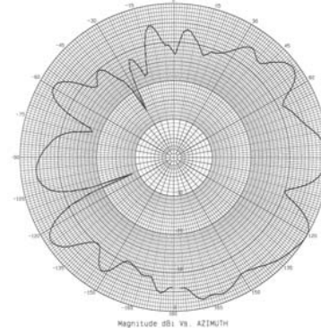
5500 MHz – Azimuth
