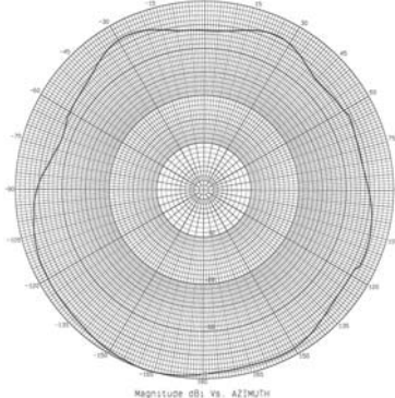
2700 MHz – Azimuth
