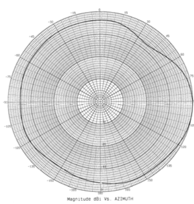
1850 MHz – Azimuth Plot
