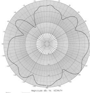
4900 MHz – Azimuth
