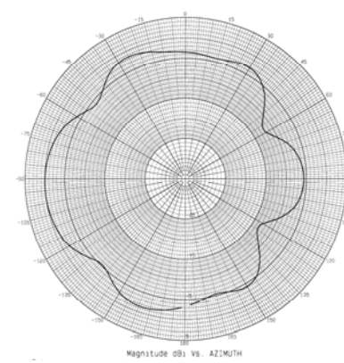
2700 MHz – Azimuth Plot
