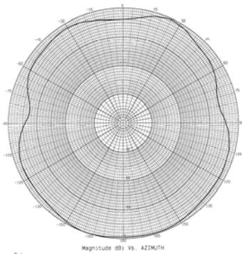
2450 MHz – Azimuth
