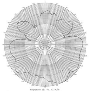
5950 MHz – Azimuth
