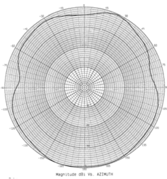
2450 MHz – Azimuth
