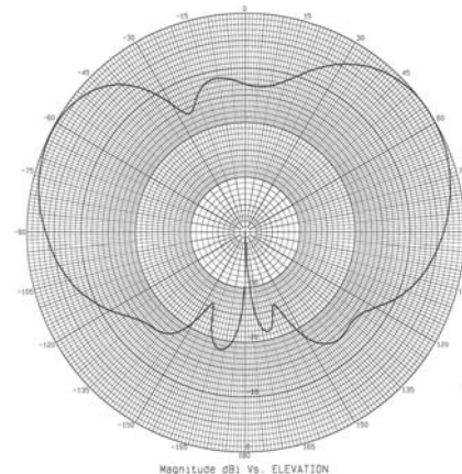
2100 MHz – Elevation Plot
