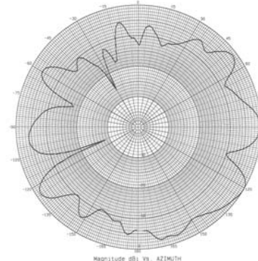
5500 MHz – Azimuth
