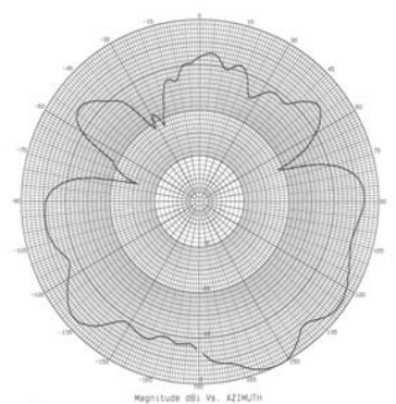
5950 MHz – Azimuth
