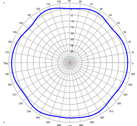
MGRM at 2400 MHz – Azimuth Plot
