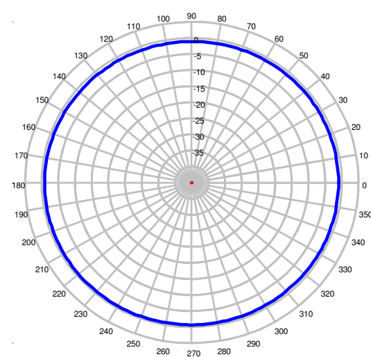
850 MHz – Azimuth Plot
