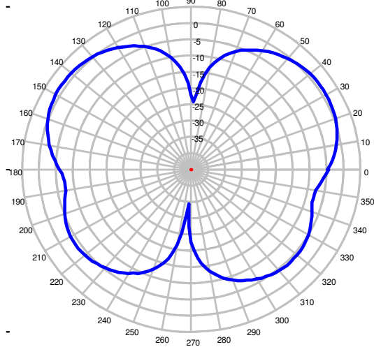
695 MHz – Elevation Plot
