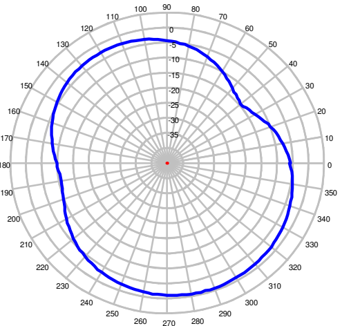
2700 MHz – Azimuth Plot
