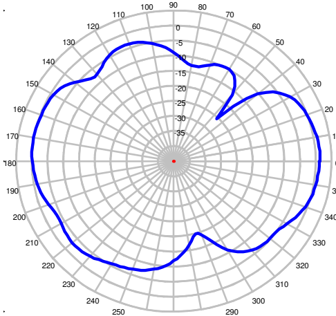
1900 MHz – Elevation Plot
