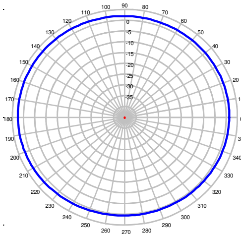
1750 MHz – Azimuth Plot
