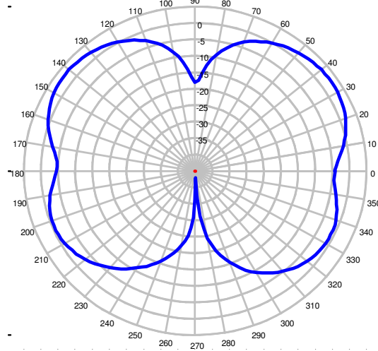
850 MHz – Elevation Plot
