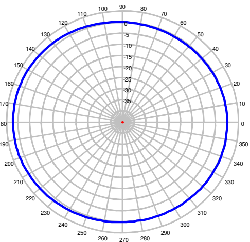
1850 MHz – Azimuth Plot
