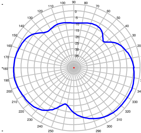
1750 MHz – Elevation Plot
