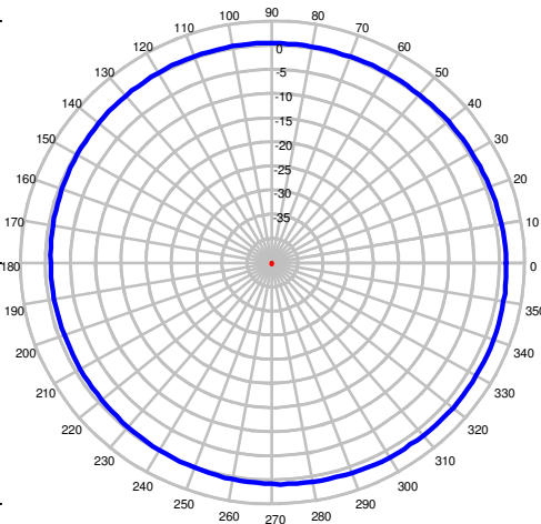
2170 MHz – Azimuth Plot
