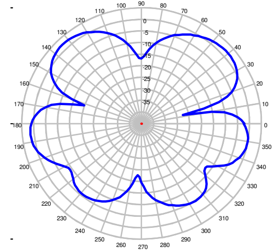
925 MHz – Elevation Plot
