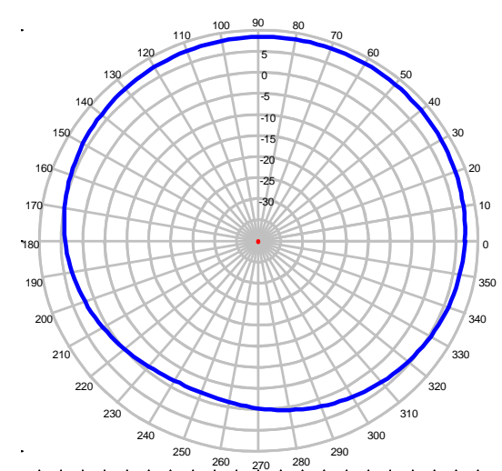
925 MHz – Azimuth Plot
