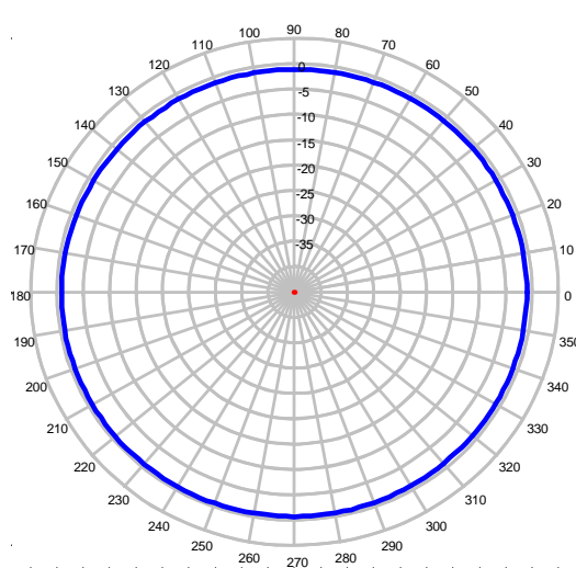
850 MHz – Azimuth Plot
