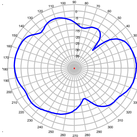
1900 MHz – Elevation Plot
