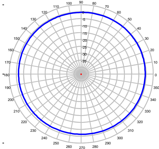
695 MHz – Azimuth Plot
