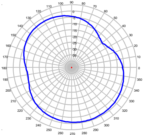
2700 MHz – Azimuth Plot
