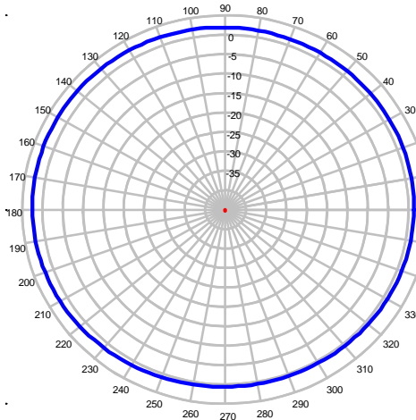
1750 MHz – Azimuth Plot
