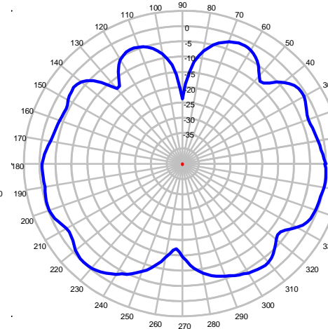
2170 MHz – Elevation Plot
