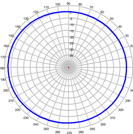
1850 MHz – Azimuth Plot
