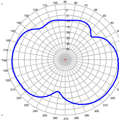
1750 MHz – Elevation Plot
