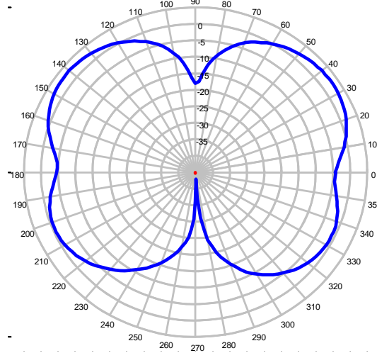
850 MHz – Elevation Plot
