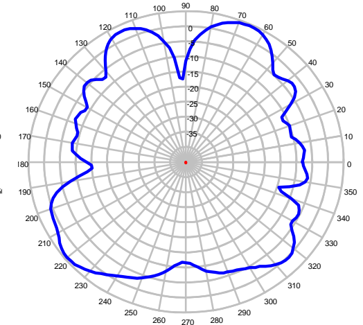
2700 MHz – Elevation Plot
