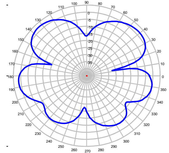
925 MHz – Elevation Plot
