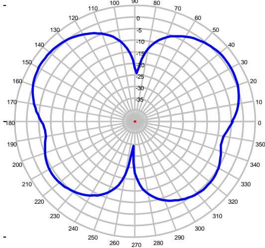
695 MHz – Elevation Plot
