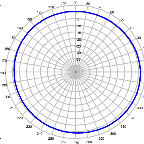
2170 MHz – Azimuth Plot
