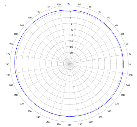
2170 MHz Azimuth Plot
