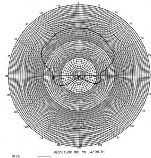
PS11-5500-90 – Azimuth Plot
