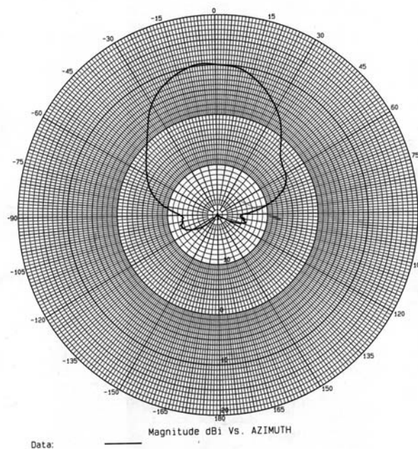
PS14-5500-45 – Azimuth Plot
