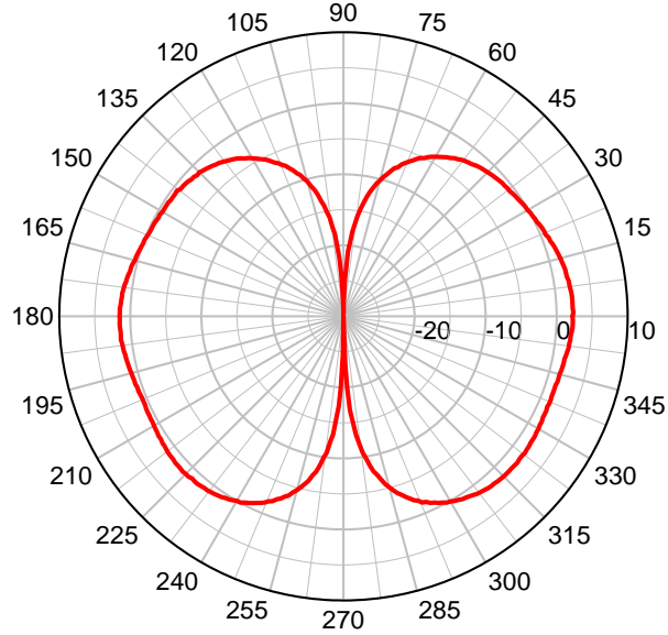
PSKN3 900S Series – Elevation Plot
