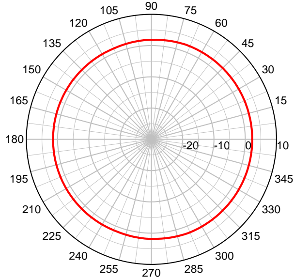
PSKN3 900S Series – Azimuth Plot
