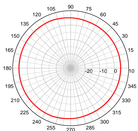
Cable #1, #2 & #3 SMW 5500 MHz – Azimuth Plot
